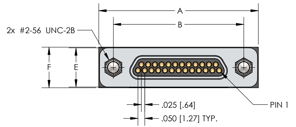
FRONT VIEW - PLUG (PINS)
