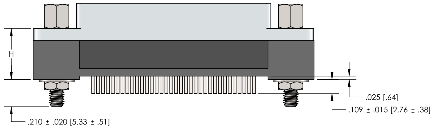
FRONT VIEW - RECEPTACLE (SOCKETS)
