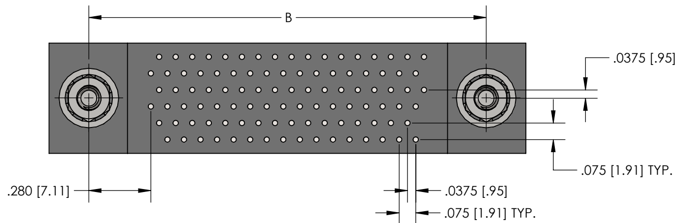
BOTTOM VIEW - RECEPTACLE SIZE 100
