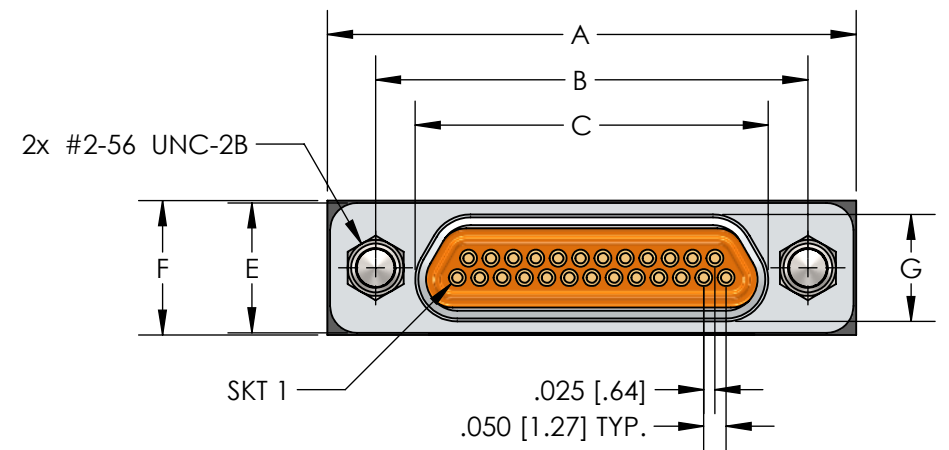
FRONT VIEW - RECEPTACLE (SOCKETS)
