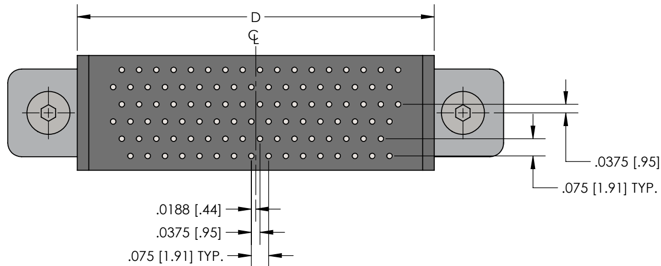
BOTTOM VIEW - RECEPTACLE SIZE 100
