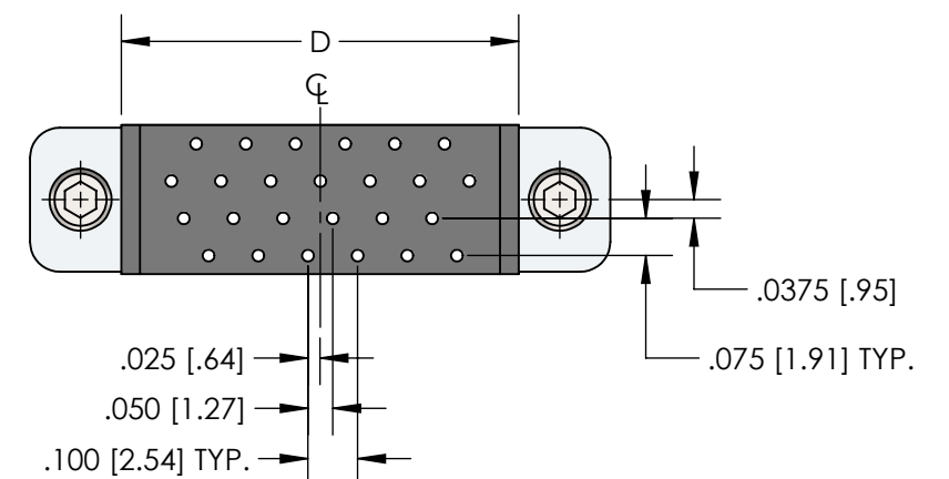
BOTTOM VIEW - RECEPTACLE SIZE 9, 15, 21, 25, 31, AND 37
