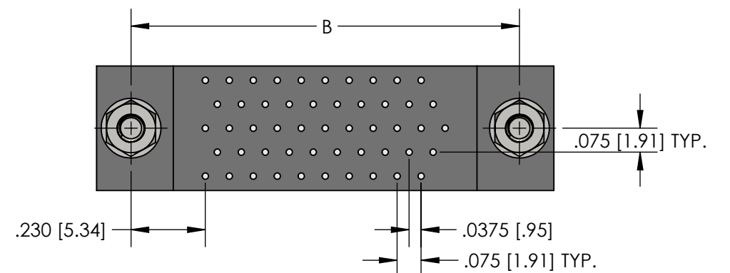
BOTTOM VIEW - RECEPTACLE SIZE 51-3
