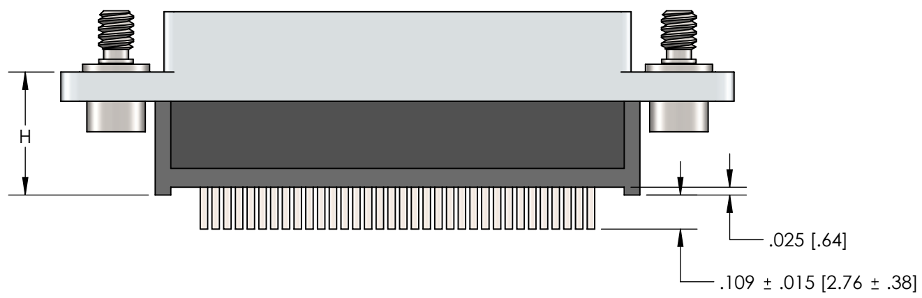
FRONT VIEW - RECEPTACLE (SOCKETS)
