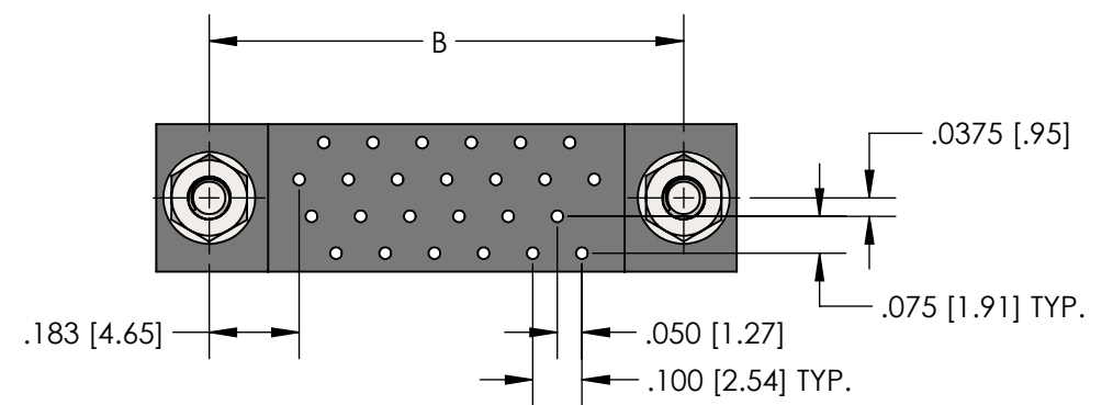
BOTTOM VIEW - RECEPTACLE SIZE 9, 15, 21, 25, 31, AND 37
